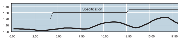
Typical SWR of a 41-10
