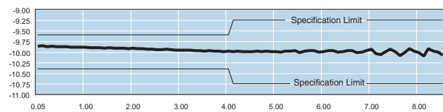
Typical Attenuation Accuracy of a 24-10-34
