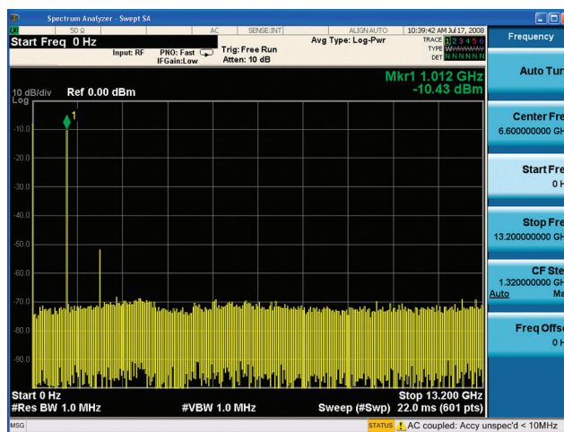
Figure 4b. The MXA only takes 22 ms for a full span of 13.2 GHz sweep (RBW=VBW=1 MHz).
