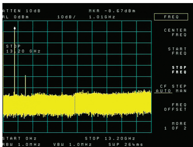
Figure 4a. The 8562 EC takes 260 ms for a full span of 13.2 GHz sweep (RBW=VBW=1 MHz).
