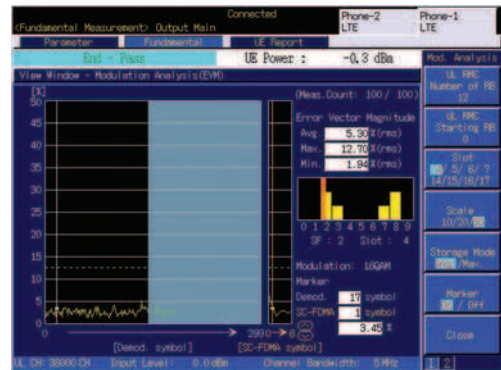
Transmitter Measurement (EVM)
