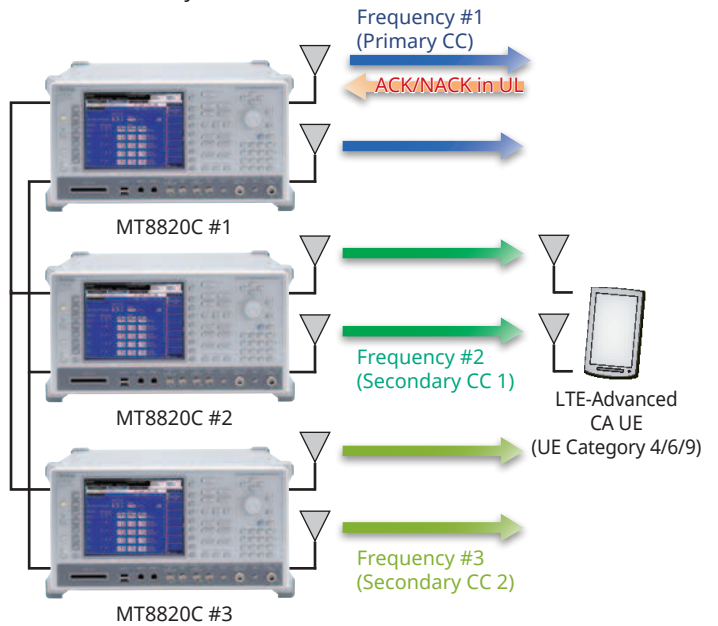
Sample MT8820C connection
