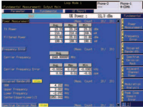
Transmitter Measurement
